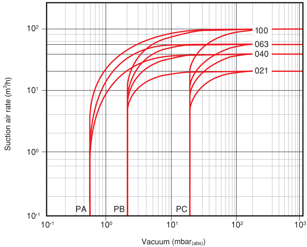
Performance Chart 50 Hz
